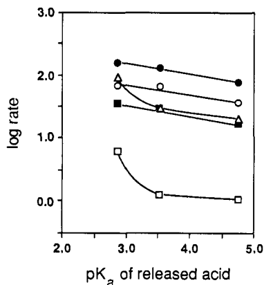
Figure 5. Effect of the pK_a of the released carboxylic acid on the rates of PKA-catalyzed hydrolysis of acylnorvaline (●), \alpha -allylglycine (○), \alpha -propargylglycine (■), -glutamic acid (Δ), and -phenylalanine (□). The pK_a values of the free acids that form the acyl groups are 2.86 (chloroacetic), 3.53 (methoxyacetic), and 4.76 (acetic).
